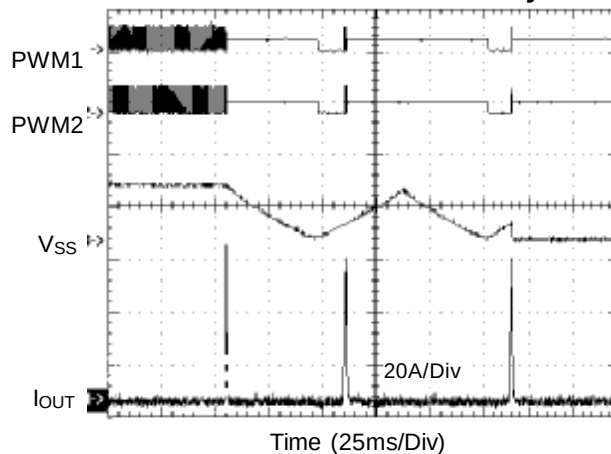
Over Current Protection at Steady State
