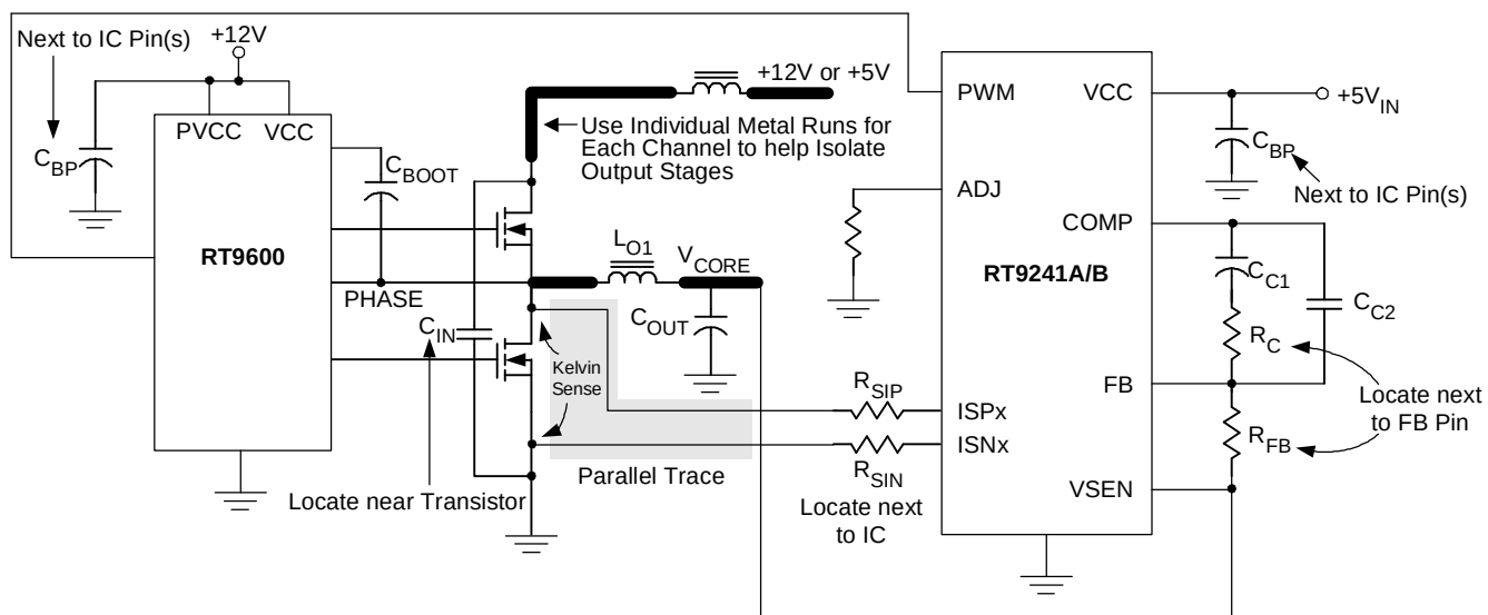
Figure.8 Layout Consideration
