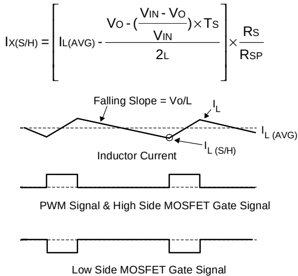
Figure 2. Inductor Current and PWM Signal
