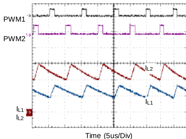
Two-Phase Converter without Current Sharing
